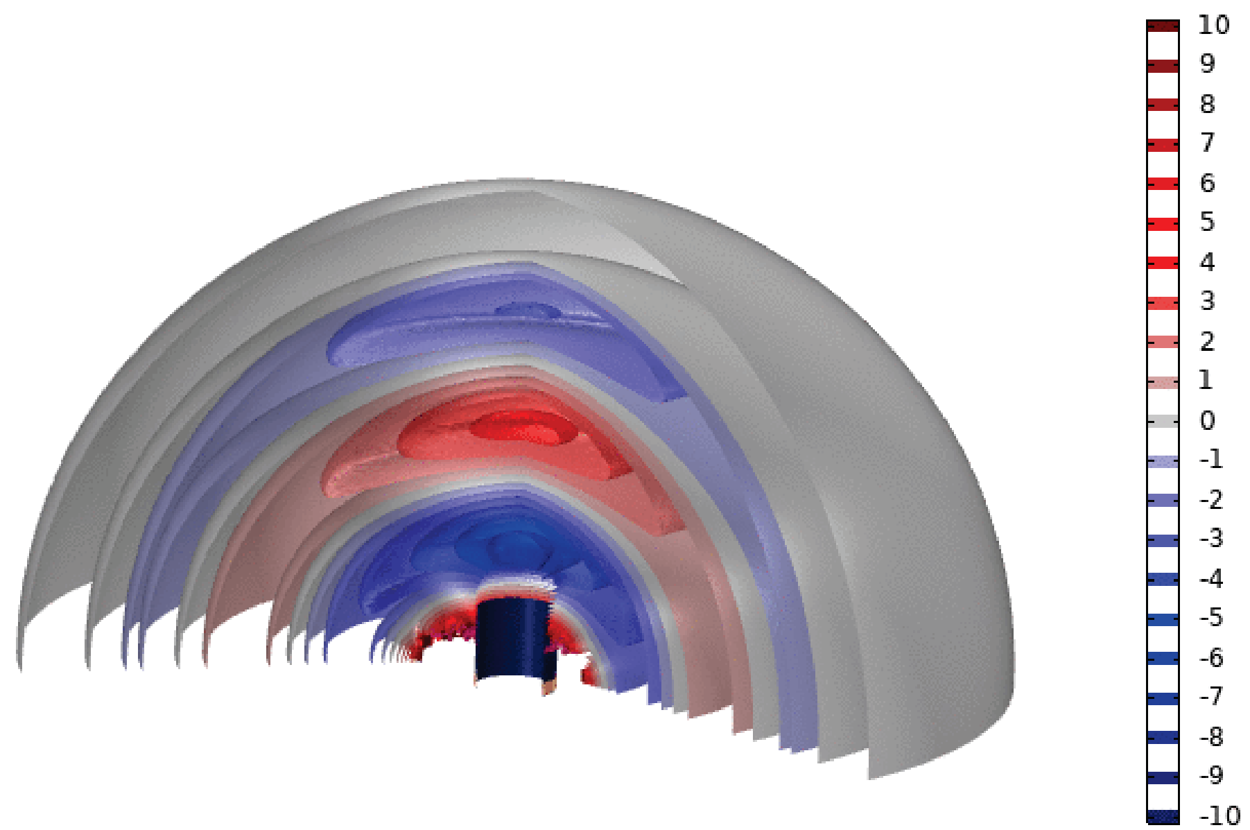
Acoustic Pressure Generated by the Spider Vibration (Pa)
